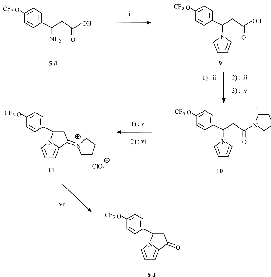
Scheme 3. (i) 2,5-diOMeTHF, AcOH; (ii) TEA, (\text{CH}_3)_2\text{CO} ; (iii) \text{ClCO}_2\text{Et} , (\text{CH}_3)_2\text{CO} ; (iv) pyrrolidine, (\text{CH}_3)_2\text{CO} ; (v) \text{POCl}_3 , toluene; (vi) \text{HClO}_4 , \text{H}_2\text{O} ; (vii) \text{NaOH} , \text{H}_2\text{O} .
