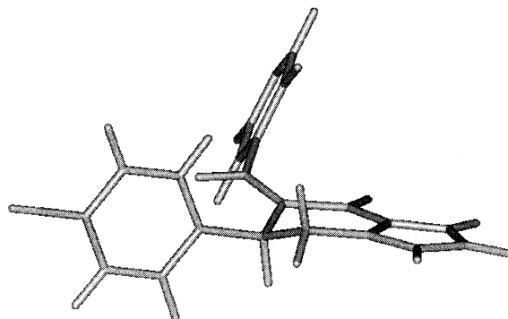
Figure 2. One equatorial conformation of compound 30 .
