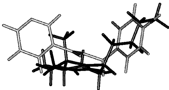
Figure 1. Superimposition of compounds 21 and 30 .
