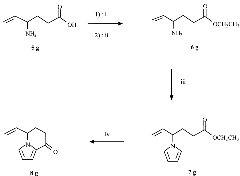
Scheme 5. (i) \text{SOCl}_2 , EtOH; (ii) \text{NH}_3 gas, EtO 2 ; (iii) 2,5-diOMeTHF, AcOH; (iv) \text{BBr}_3 , \text{CH}_2\text{Cl}_2 .
